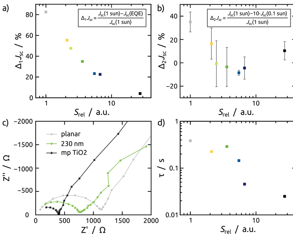
Figure 6. Time scales for ion migration in perovskite cells featuring various specific surface areas S_{\text{rel}} . (a) Relative difference \Delta_1 J_{\text{sc}} between short circuit current densities determined (1) by integrating the EQE spectrum measured without bias light under 30 Hz chopped single-wavelength irradiation ( J_{\text{sc}}(\text{EQE}) ) and (2) under steady-state 1 sun white light irradiation ( J_{\text{sc}}(1 \text{ sun}) ). (b) A similar analysis using J_{\text{sc}} values recorded in high- and low-light conditions confirms that the trend is physically meaningful. (c) Impedance spectroscopy: exemplary set of Nyquist plots recorded at J_{\text{sc}} and 0.5 sun on three samples. (d) Evolution of characteristic times extracted from impedance spectroscopy data sets, which follow the same trend and confirm its origin in ionic transport.
